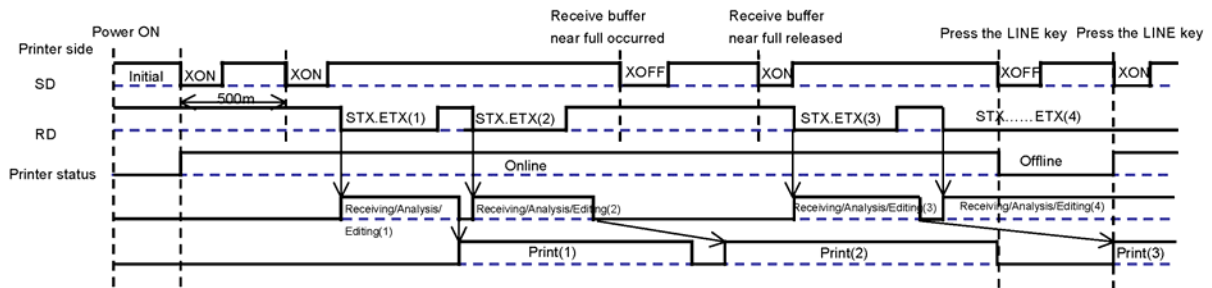
(1) Normal process
